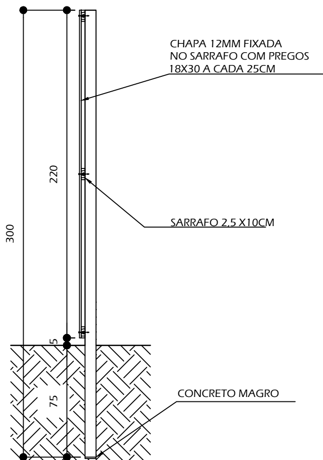
VISTA FRONTAL
