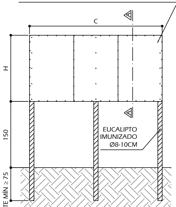
VISTA FRONTAL
