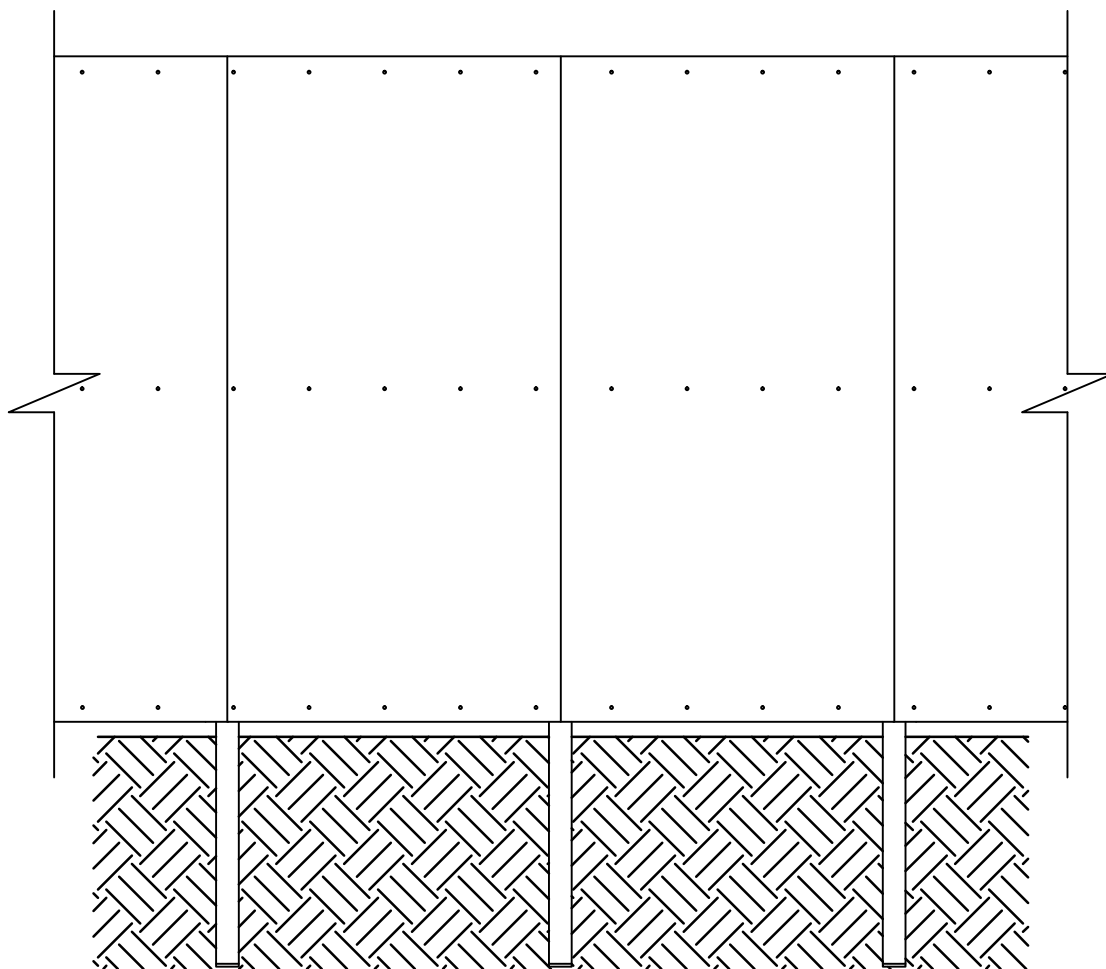
VISTA FRONTAL
